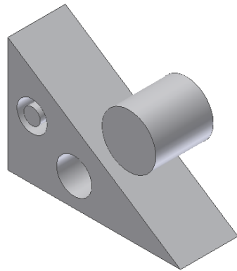
Combine = True
