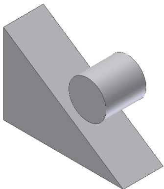
Combine = False
